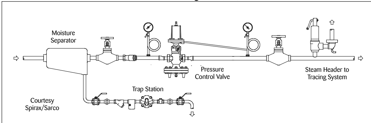
Figure 6 Steam Pressure Reducing Valve (PRV) Station
