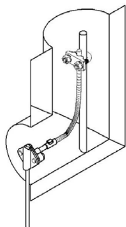
TYPICAL EBP2P-08-T
