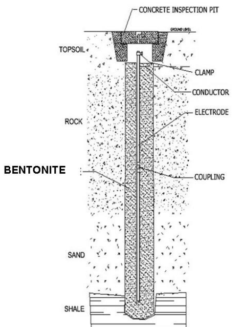
TYPICAL ELECTRODE INSTALLATION
