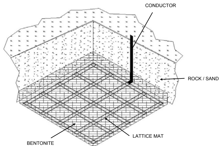
TYPICAL LATTICE MAT INSTALLATION
