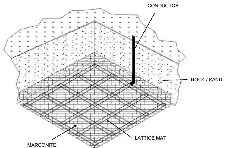
TYPICAL LATTICE MAT INSTALLATION
